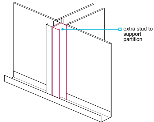
Figure 22: Partitioning abutment
