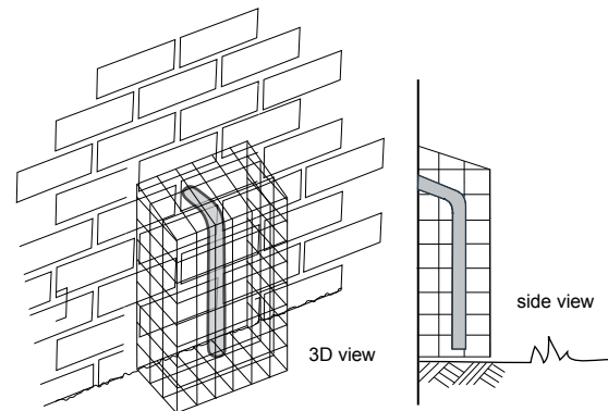
Figure 17: Low-level unvented discharge — path or garden area
