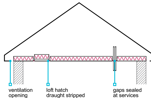
Figure 56: Ceiling penetrations
