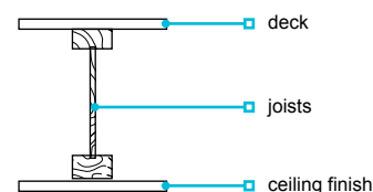
Figure 5: Uninsulated roof deck construction
