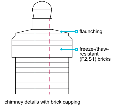
Figure 39: Chimney details with brick capping
