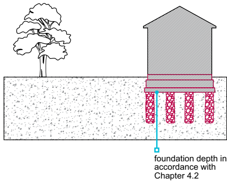
Figure 3: Vibro foundation depth in volume change potential soils
