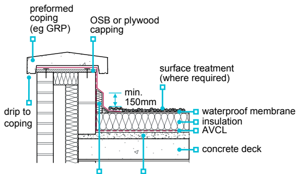
Figure 32: Upstands
