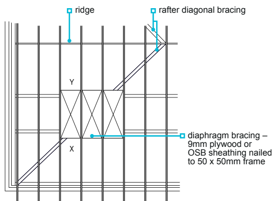
Figure 34: Attic truss — diaphragm bracing
