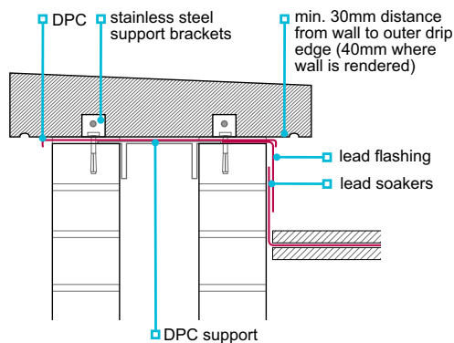
Figure 74: Raking coping — masonry
