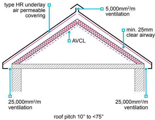
Figure 48: Warm roof
