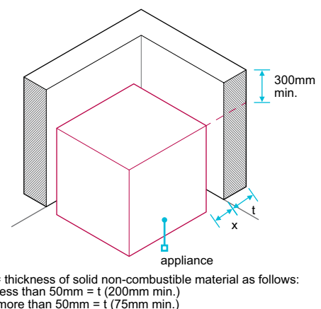
Figure 3: Solid fuel appliance clearances to wall
