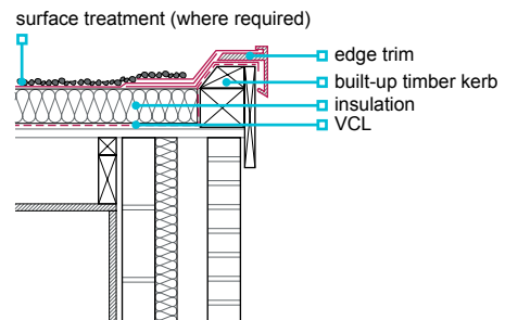
Figure 38: Verge detail
