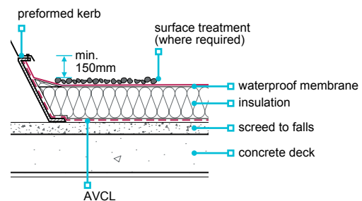
Figure 33: Skirting to rooflights or ventilator kerb
