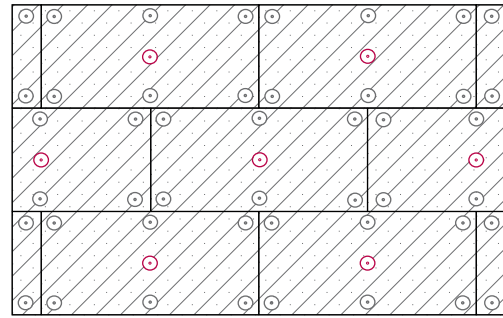
Figure 6: Insulated render with drained cavity
