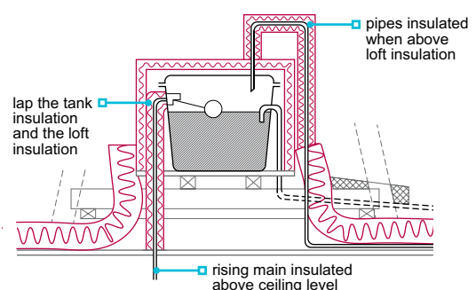
Figure 57: Storage tank insulation
