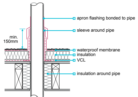
Figure 40: Pipe passing through roof
