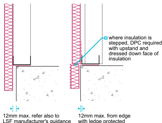
Figure 9: Floor edges
