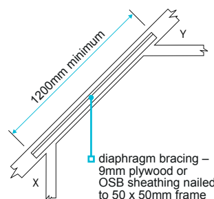
Figure 35: Attic truss — diaphragm bracing
