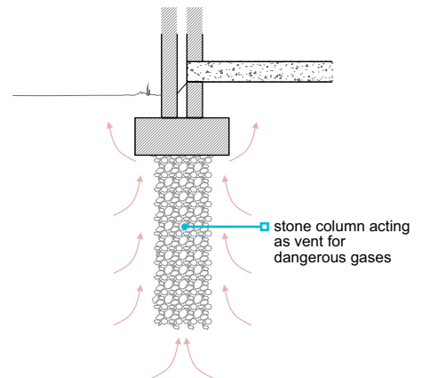
Figure 2: Stone column acting as vertical vent
