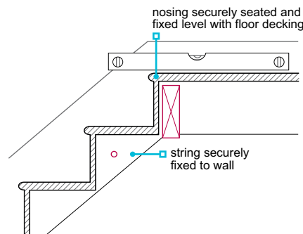
Figure 16: Staircase fixing
