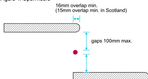
Figure 4: Open risers
