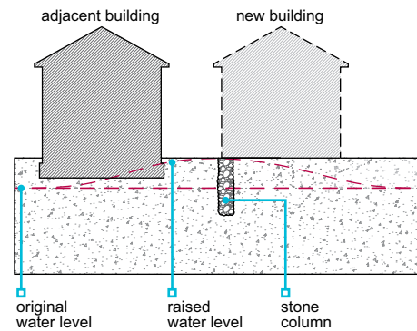
Figure 7: Effect of raised water level on adjacent building
