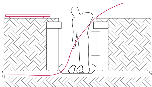
Figure 4: Manhole
