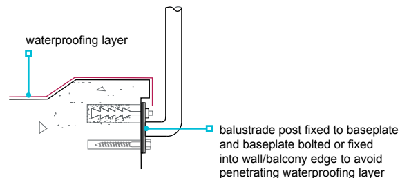
Figure 52: Balustrade post fixed to wall below coping/kerb
