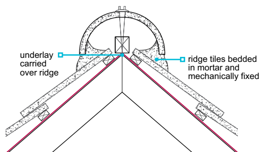
Figure 64: Wet bedded ridge with dentil tiles
