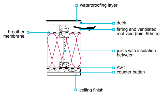
Figure 3: Cold roof
