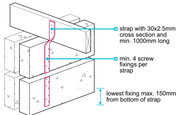
Figure 15: Joist strap
