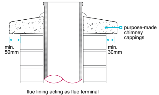
Figure 6: Chimney capping
