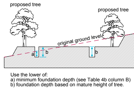
Figure 7: Levels from which foundation depths are measured where trees or hedgerows are proposed
