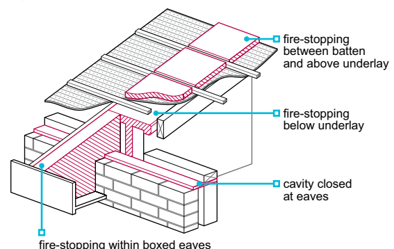
Figure 9: Junction of compartment wall and roof
