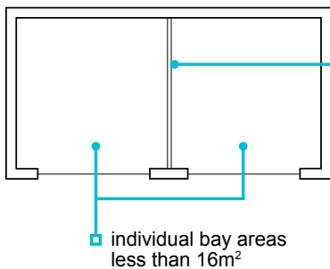
Examples of unreinforced concrete floors in garages where the total floor area exceeds 16m 2
