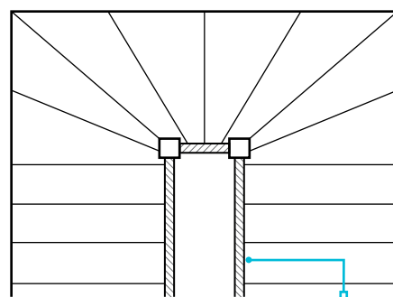
Figure 14: Handrail provision
