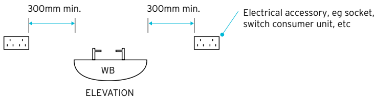
Diagram 1 - wash basin
