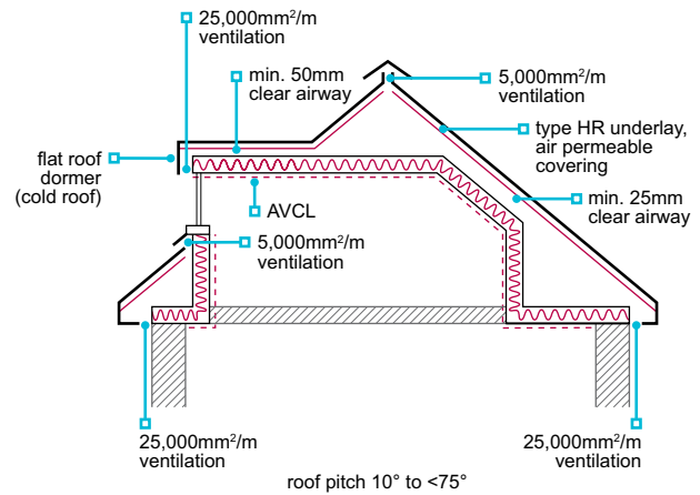
Figure 47: Hybrid roof — Room-in-roof (flat roof dormer)
