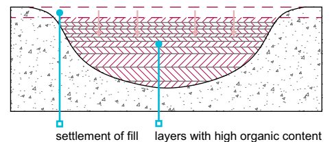
Figure 1: Ground subject to settlement
