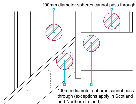
Figure 7: Protective guarding
