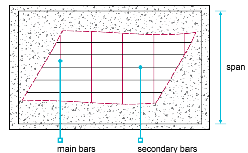
Figure 2: Reinforcement layout
