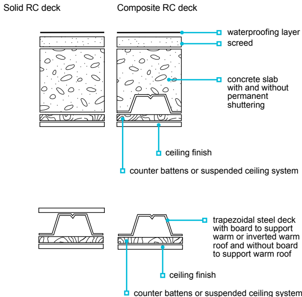
Figure 4: Inverted warm roof
