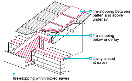
Figure 58: Fire precautions
