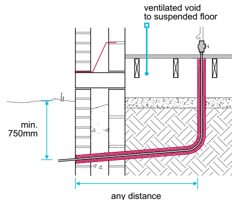
Figure 4: Underfloor water supply pipe insulation
