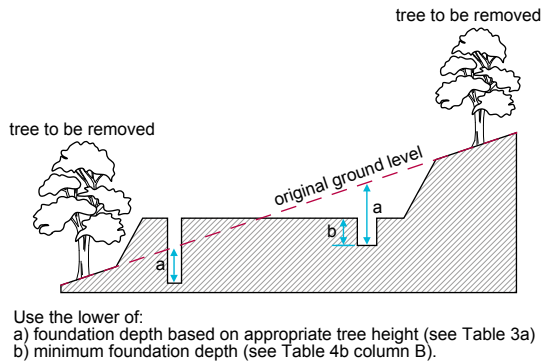
Figure 6: Levels from which foundation depths are measured where trees or hedgerows are removed
