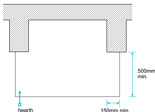
Figure 16: Hearth clearances
