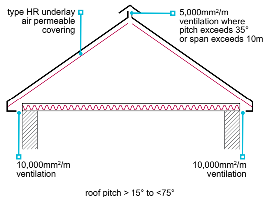
Figure 44: Roof pitch >15° and <75°
