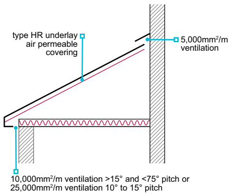
Figure 45: Mono pitched roof
