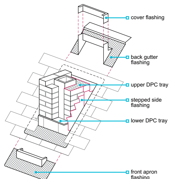
Figure 73: Chimney penetration
